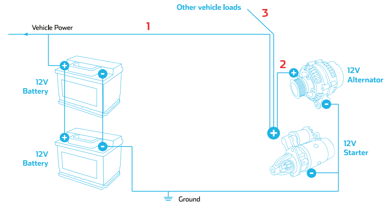
Fig 2. 12V system before SkelStart™ installation
